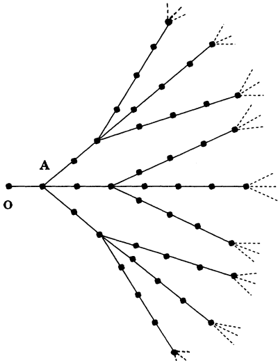
FIG. 1. An \text{NT}_D with r=3 ( D=d_f=\bar{d}=1+\log r/\log 2 ).
